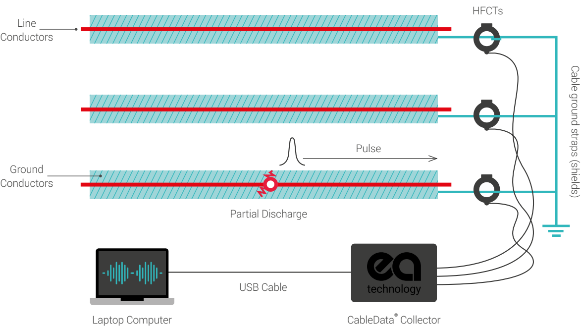
Figure 1: Setup for three phase data capture
