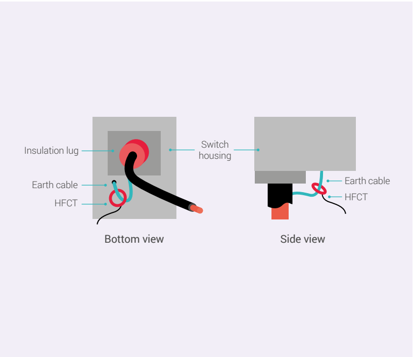
Figure 3: HFCT Connections
