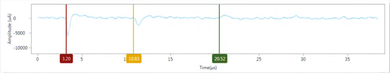
Waveform showing PD location at 56% from the measurement position.
