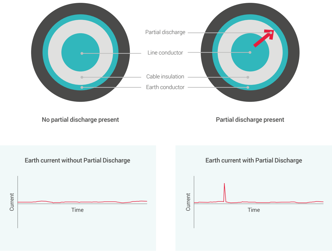
Figure 7: Effect of Partial Discharge on a cable
