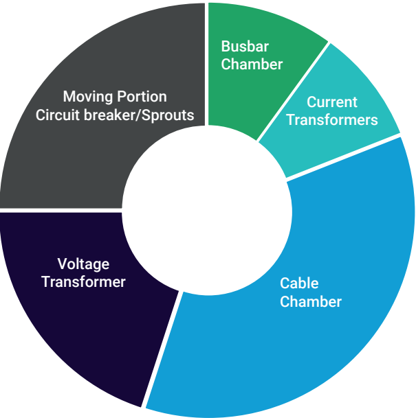
Where PD is typically found in Switchgear
